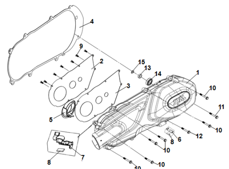
E08 L. CRANK CASE COVER
